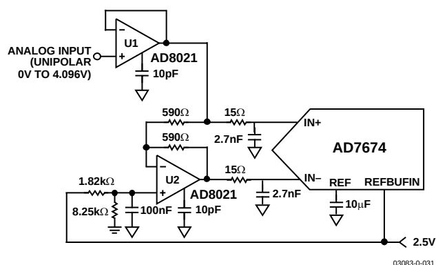
Figure 32. Single-Ended-to-Differential Driver Circuit (Internal Reference Buffer Used)
