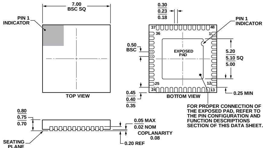
Figure 48. 48-Lead Lead Frame Chip Scale Package [LF CSP] 7 mm × 7 mm Body and 0.75 mm Package Height (CP-48-4)
