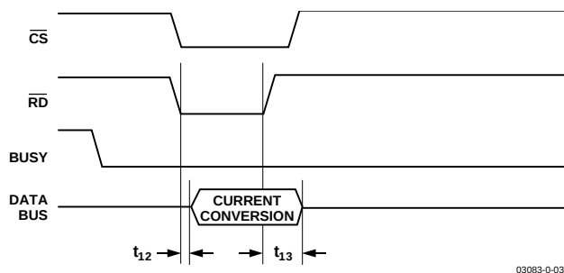
Figure 38. Slave Parallel Data Timing for Reading (Read After Convert)
